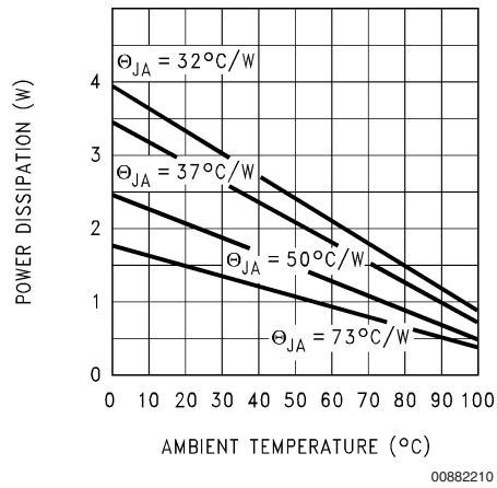
Maximum Power Dissipation (TO-263) See (Note 2)
