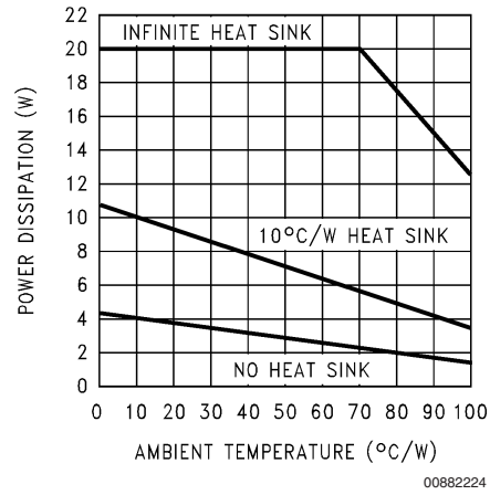
Maximum Power Dissipation (TO-3)
